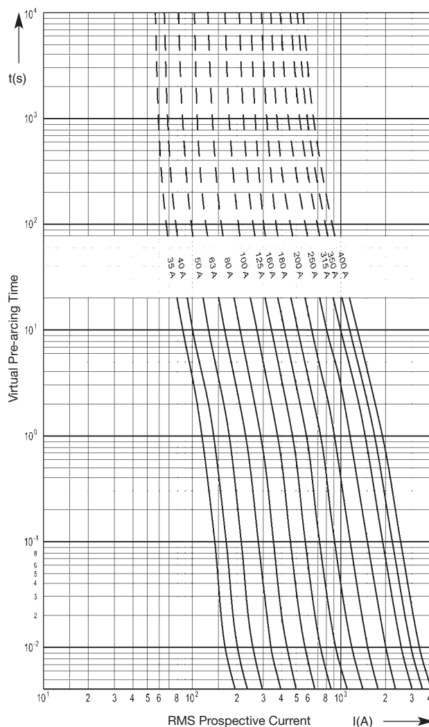
Time-Current Characteristics
